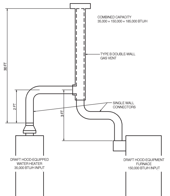
FIGURE C-B-17 (EXAMPLE 4) COMMON VENTING TWO DRAFT- HOOD-EQUIPPED APPLIANCES
