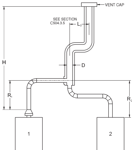
FIGURE C-B-10 ASBESTOS CEMENT TYPE B OR SINGLE-WALL METAL VENT SYSTEM SERVING TWO OR MORE DRAFT-HOOD-EQUIPPED APPLIANCES
