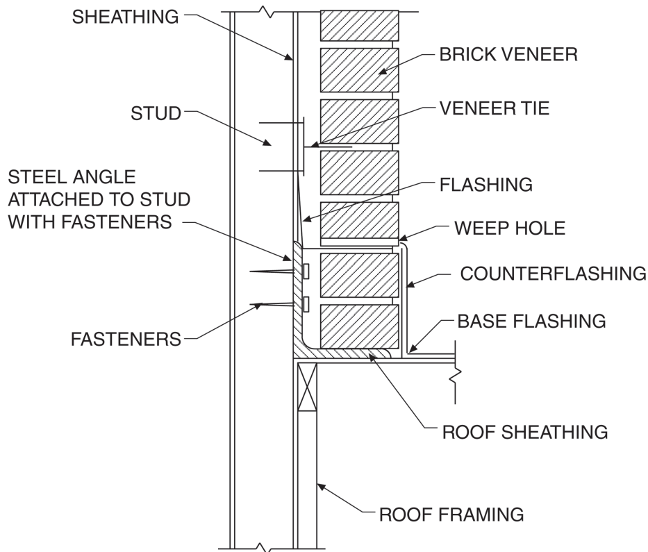
SUPPORT BY STEEL ANGLE
