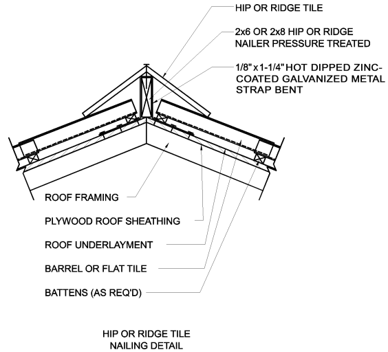
DRAWING 15 RIDGE BLOCKING DETAIL
