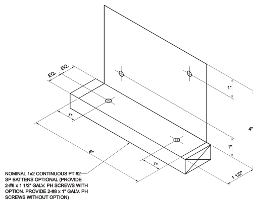
SHEET PLATE DETAIL
