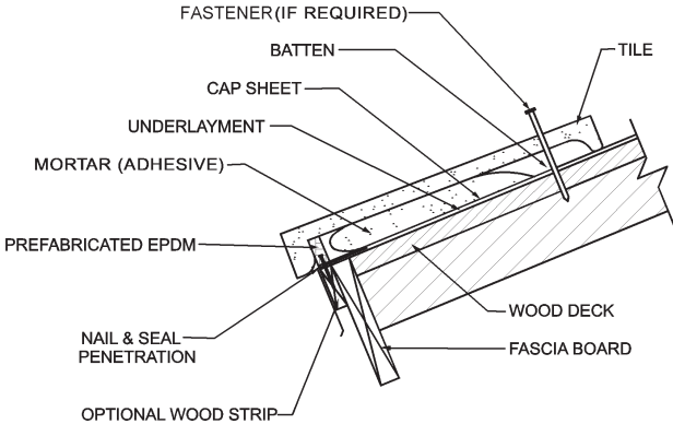
DRAWING 12 EAVE TILE DETAIL ANTIPONDING METAL
