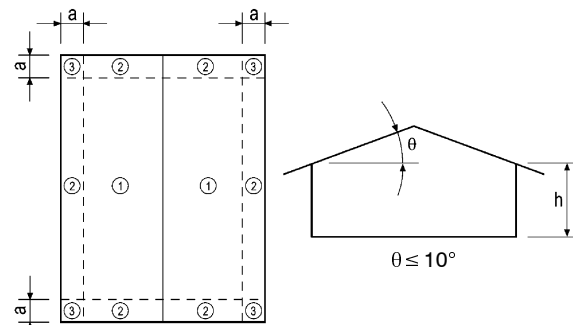
GABLE ROOFS \theta \leq 10^\circ
