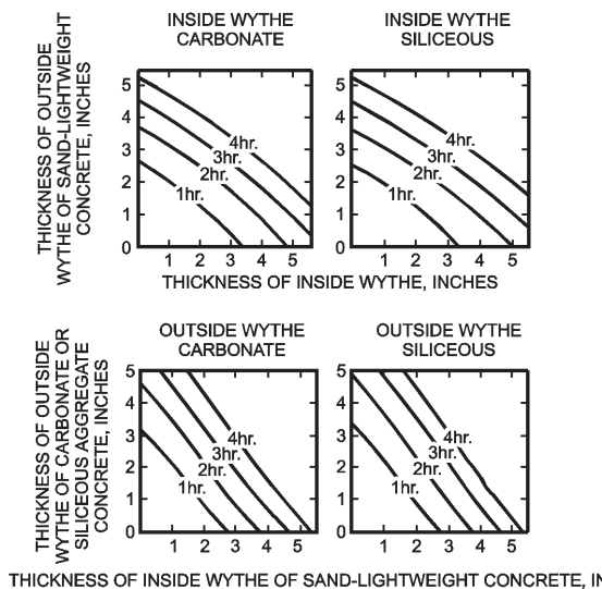
FIGURE 721.2.1.2 FIRE-RESISTANCE RATINGS OF TWO-WYTHE CONCRETE WALLS
